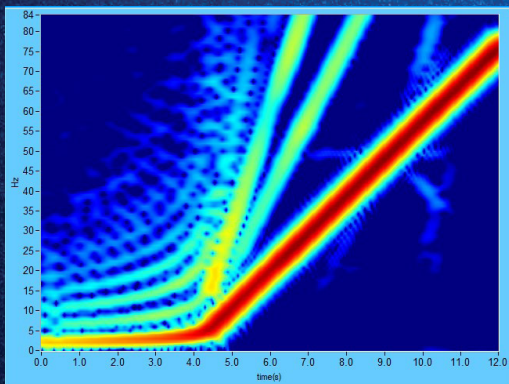
Spectral Analysis with Standard Valve (0 to -54dB)
