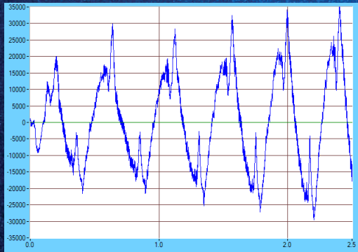
Ground Force signal with Standard Valve
