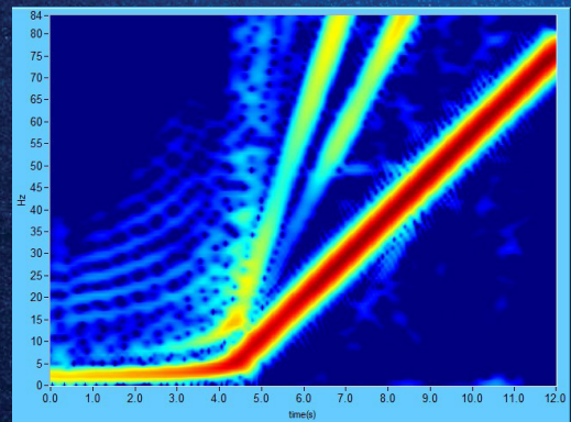
Spectral Analysis with DR3 Valve (0 to -54dB)
