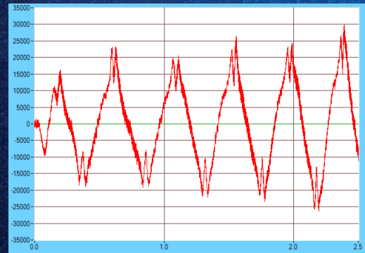
Ground Force signal with DR3 Valve
